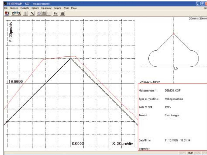
Standardized representation of a free-form test with a KGM and detail zoom: here a normal view shows an overshoot with the resulting rounding-off error. (Nominal path in black, actual path in red)
