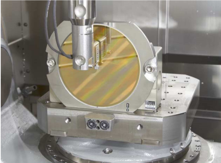
2-D measurement with KGM 181 in the XZ plane
