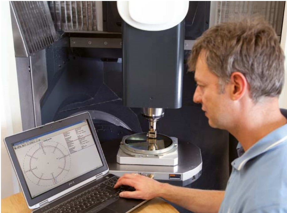
Free-form test with KGM 182
