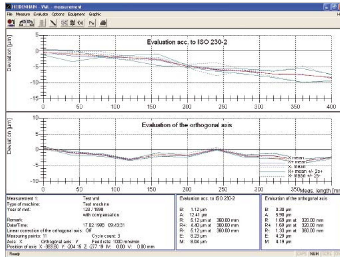
Measurement of the static positioning accuracy as per DIN ISO 230-2 and the guideway error in transverse direction with the VM 182
