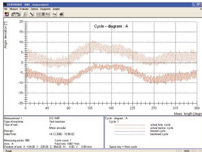
Measurement of the static positioning accuracy of a rotary table with worm gear with the RON 905 and feedback via the rotary encoder in the motor (Semi-Closed Loop) ...
